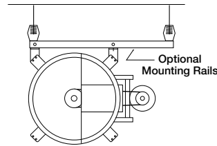
Horizontal Ceiling Hung Motor at 3 or 9 O'clock Position Fig. 4
