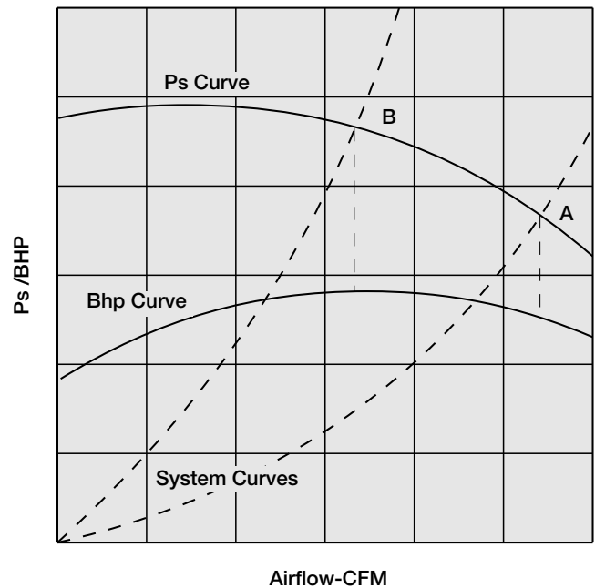
Centrifugal Fan with Outlet Damper
