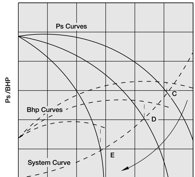
Centrifugal Fan with Inlet Damper
