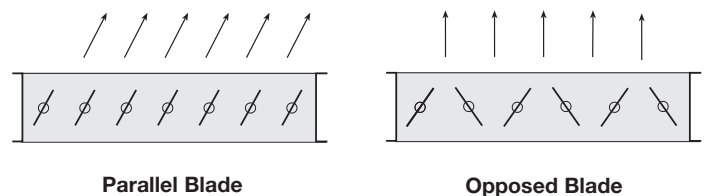
Top View of Blade Action Styles
