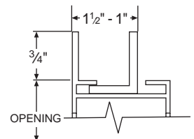
GLAZING FRAME
